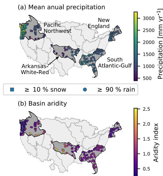
Figure 5. Overview of the location of the four hydrological units from the CAMELS data set used in this study, including all their basins. Panel (a) shows the mean annual precipitation of each basin, whereas the type of marker symbolizes the snow influence of the basin. Panel (b) shows the aridity index of each basin, calculated as PET/P (see Addor et al., 2017a).
