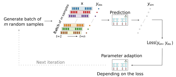
Figure 3. Illustration of one iteration step in the training process of the LSTM. A random batch of input data x consisting of m independent training samples (depicted by the colours) is used in each step. Each training sample consists of n days of look-back data and one target value ( y_{\text{obs}} ) to predict. The loss is computed from the observed discharge and the network’s predictions y_{\text{sim}} and is used to update the network parameters.
