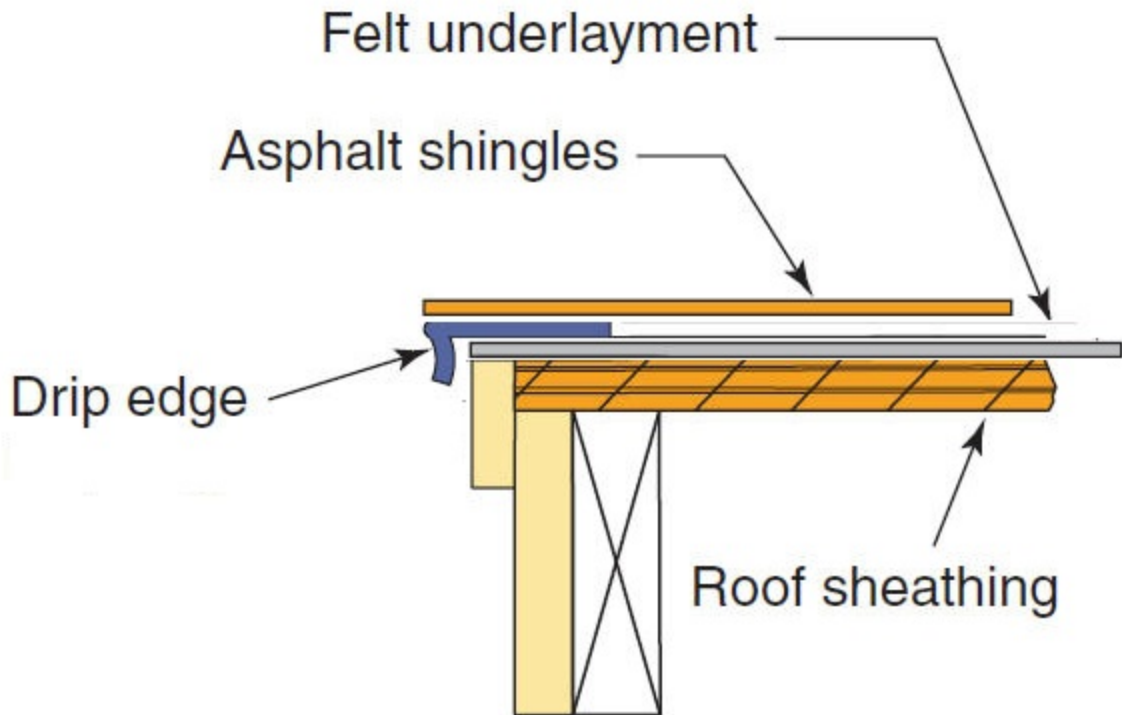
Section at rake
