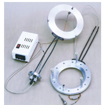
Heated annular rings with PID controller for plasma chamber
