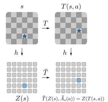
Figure 1: Visualization of the notion of equivariance under actions. We say Z is an action equivariant mapping if Z(T(s, a)) = \hat{T}(Z(s), \bar{A}_s(a)) .
