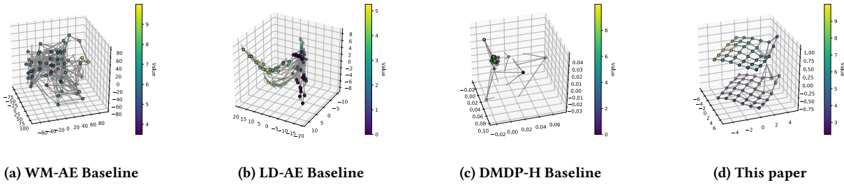
Figure 3: Abstract MDP for three approaches in the single object room domain. Nodes are PCA projections of abstract states, edges are predicted \bar{T}_\phi , colors are predicted values.
