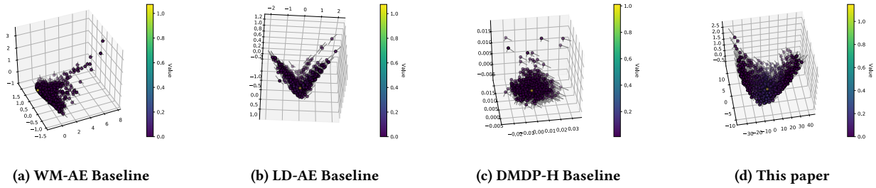
Figure 6: Abstract MDP for four approaches in CartPole. Nodes are PCA projections of abstract states, edges are predicted \bar{T}_\phi , colors are predicted values.
