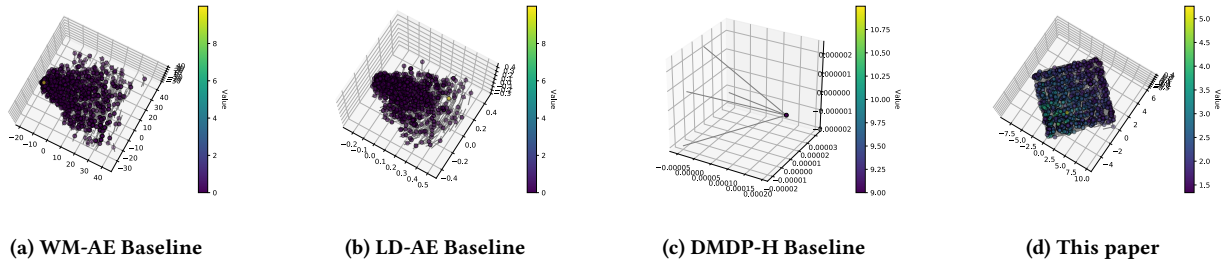
Figure 7: Abstract MDP for four approaches in planning in Fashion MNIST. Nodes are PCA projections of abstract states, edges are predicted \bar{T}_\phi , colors are predicted values.
