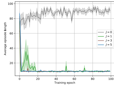
(a) Comparison of different values of J .
