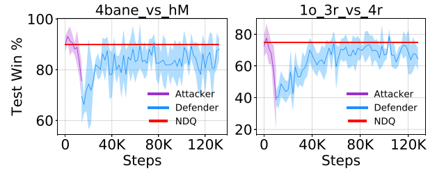
Figure 7: Multiple attackers: Attack and defence on NDQ.
