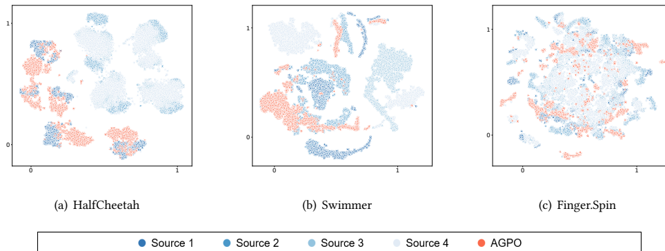
Figure 6: t-SNE graph of expert demonstrations (blue) and samples generated by our method (orange) on three tasks. Samples generated by our methods demonstrate high similarity with high-quality samples.
