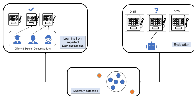
Figure 1: Overview of the methodology of our approach. Most of the off-the-shelf exploration methods can be generalized to the anomaly detection process, and this process can be used to solve the learning from imperfect demonstrations problem.
