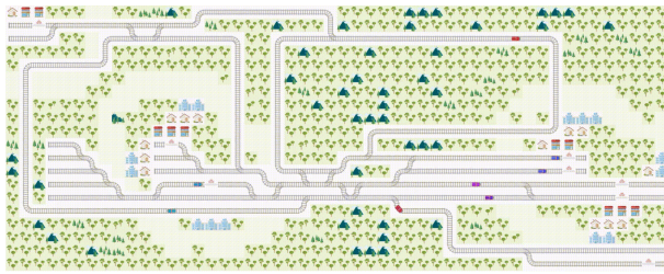
(a) Flatland
