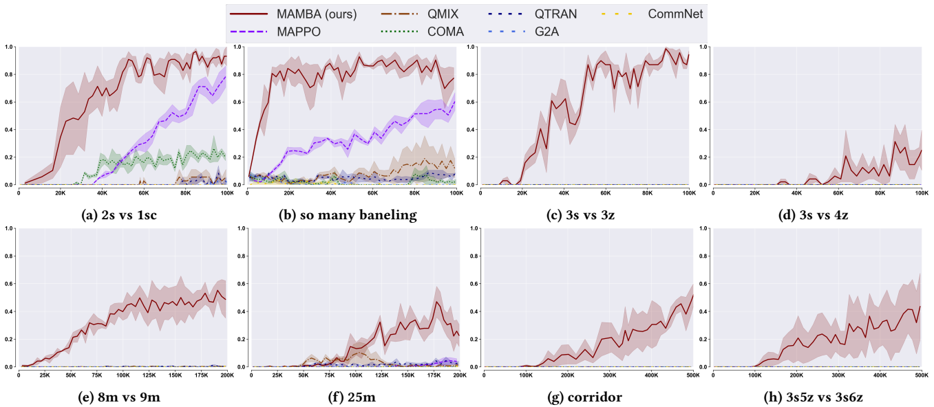
Figure 4: Experiments in SMAC environments. Y axis denotes winning rate of the agents and X axis denotes number of steps taken in the environment.
