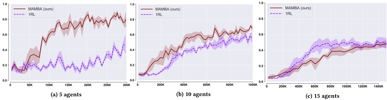
Figure 5: Experiments in Flatland environment. Y axis denotes percentage of arrived trains and X axis denotes number of steps taken in the environment.
