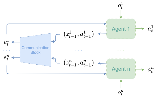
Figure 2: Execution Phase. Each agent has its own version of the world model, which can be updated using the Communication Block. It is sufficient to send only stochastic state z_{t-1}^i and action a_{t-1}^i from the previous step for each agent in order to obtain feature vectors e_t^i . Agent i then can use the updated world model and its current observation o_t^i to output its next action a_t^i .
