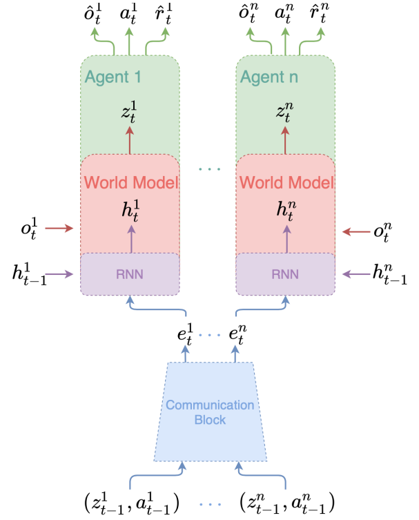
Figure 1: Training Phase. Transitions (o_{t-1}^i, a_{t-1}^i, o_t^i) are sampled from the buffer. Agents use the Communication Block to predict their current state feature vectors e_t^i from stochastic states and actions from previous step (z_{t-1}^i, a_{t-1}^i) . These feature vectors are then used to update the hidden state of the model h_t^i . Agent then can predict current stochastic state z_t^i from h_t^i and its current observation o_t^i and in turn use it to predict local information such as observation \hat{o}_t^i and reward \hat{r}_t^i . Agent also uses stochastic state to predict its next action a_t^i . During the imaginary rollout stage, Communication Block utilizes predicted stochastic states \hat{z}_t^i instead of z_t^i and observations o_t^i are not used.
