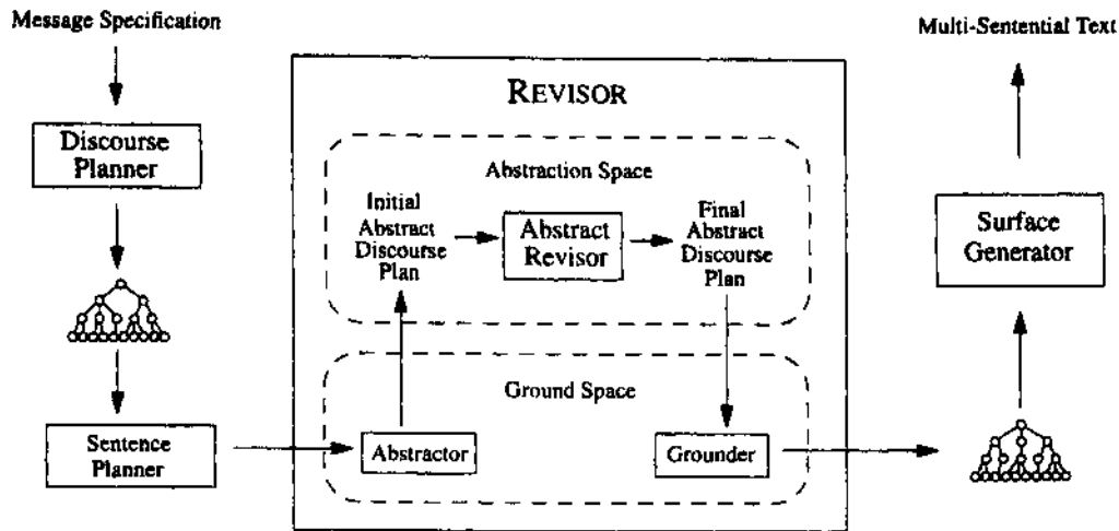
Figure 3: The revision-based explanation architecture
