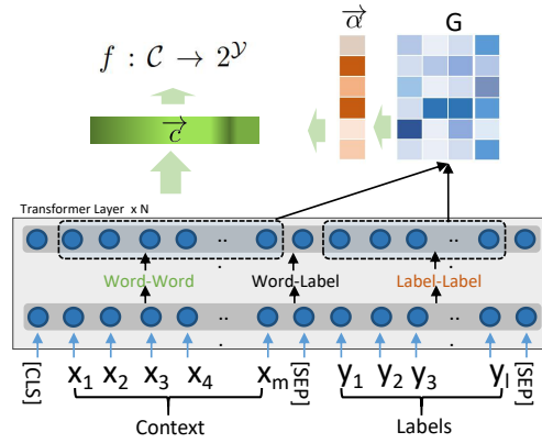
Figure 1: The framework of CORE. Specifically, word and label representations are first generated by a multi-layer Transformer encoder, which learns effectively about word-word, word-label, and label-label correlations through self-attention. After that, we focus on learning context-label correlation matrix by the output representations. Text representation vector is generated by the part of context output and attention vector, which is finally used to predict labels.
