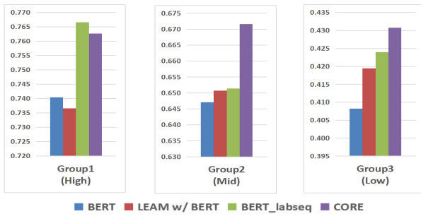
Figure 3: Macro-F1 for three groups on AAPD. All classes are sorted in descending order of their frequency of occurrence. Group1, Group2, and Group3 denote high-frequency labels, mid-frequency labels, and low-frequency labels, respectively.
