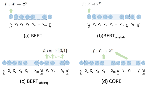
Figure 2: Illustration of different BERT-based methods. Subfigure(a) corresponds to the classical BERT of the classification task. Subfigure(b) represents a label embedding method that does not consider label correlations, corresponding to BERT onelab . Subfigure(c) uses the label-related parts of the context-label representations, corresponding to BERT labseq . Subfigure(d) is a simplified diagram of Figure 1, corresponding to CORE .
