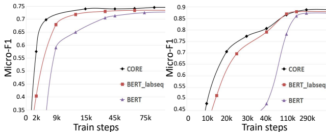
(a) Convergence speed of AAPD (b) Convergence speed of RCV1-V2 Figure 4: The convergence speed of three BERT-based methods. The x-axis refers to the training steps, and the y-axis refers to the micro-F1 score performance.
