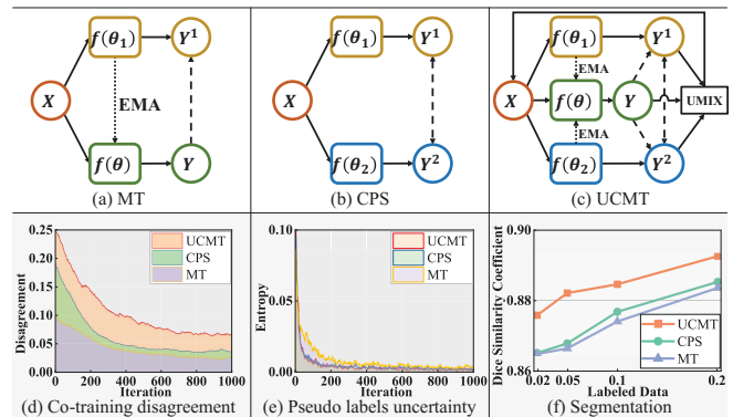
Figure 1: Illustration of the architectures and curves for co-training based semi-supervised semantic segmentation. (a) Mean-teacher [Tarvainen and Valpola, 2017], (b) Cross pseudo supervision [Chen et al. , 2021], (c) Uncertainty-guided collaborative mean-teacher, (d) the disagreement variation between the co-training sub-networks in terms of dice loss ( w.r.t. number of iterations) of two branches ( Y^1 and Y in MT; Y^1 and Y^2 in CPS; Y^1 and Y^2 in UCMT), (e) the uncertainty variation of the pseudo labels in terms of entropy w.r.t. number of iterations, and (f) the performance of MT, CPS, and UCMT on semi-supervised skin lesion segmentation under different ratio of labeled data. EMA: exponential moving average.
