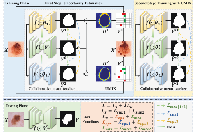
Figure 2: Overview of the proposed UCMT. CMT includes three sub-networks, i.e., the teacher sub-network ( f(\cdot; \theta) ) and the two student sub-networks ( f(\cdot; \theta_1) and f(\cdot; \theta_2) ). UMIX constructs each new samples X' by replacing the top k most uncertain regions (red grids in V^1 and V^2 ) with the top k most certain regions (green grids in V^2 and V^1 ) in the original image X .
