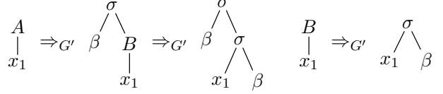
Figure 5: The relevant derivations using only productions that are not \Delta -lexicalized (see Example 14).
