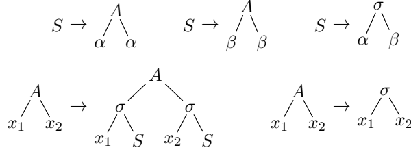
Figure 3: Productions of Example 2.
