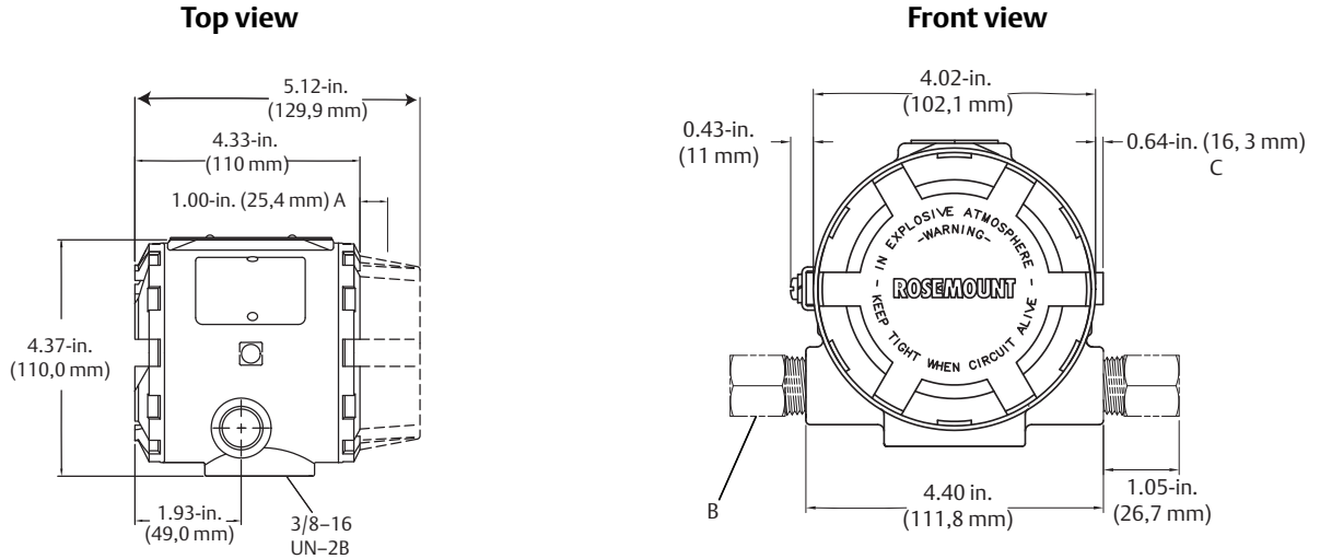
Figure 4. Transmitter for Conduits with M20 × 1.5, PG 13.5 Entries
