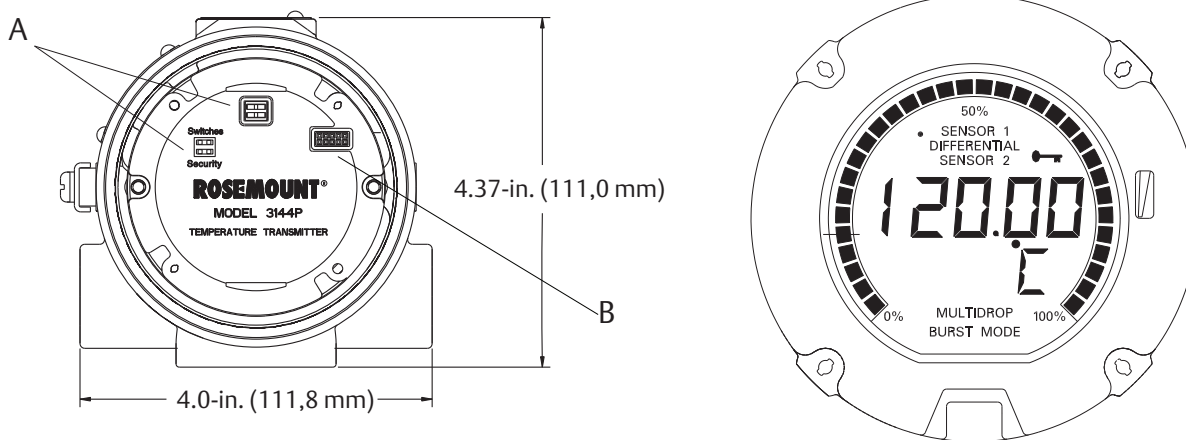
Figure 2. Switch Location and LCD Display Faceplate
