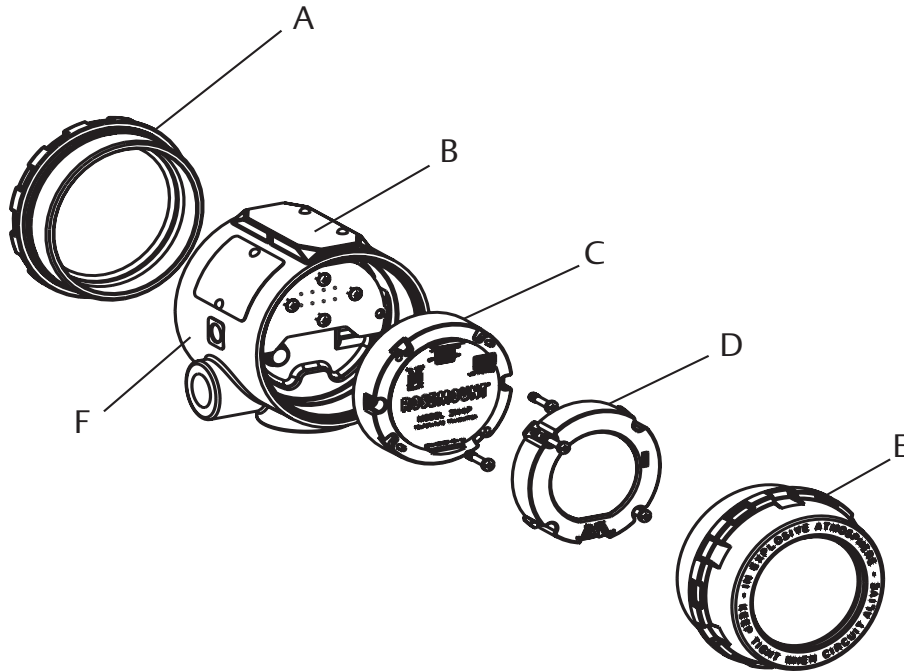
Figure 1. Transmitter Exploded View
