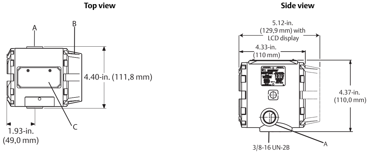
Figure 3. Transmitter
