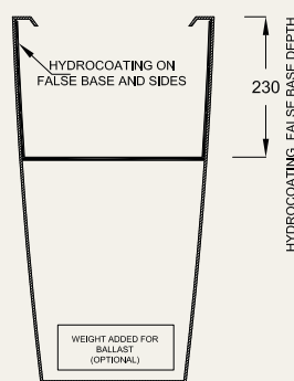
Example standard Hydroculture false base
