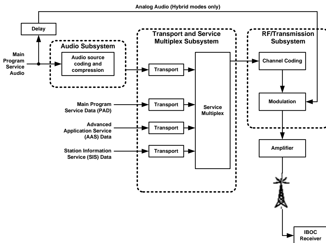
FIGURE 7 IBOC digital radio broadcasting model
