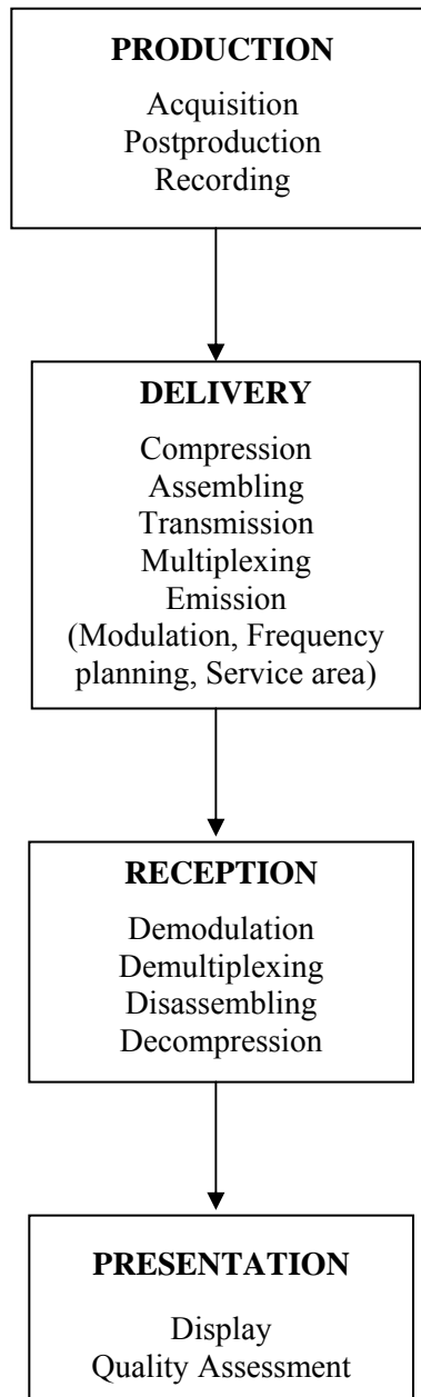
FIGURE 1 Conceptual block diagram of the broadcasting chain
