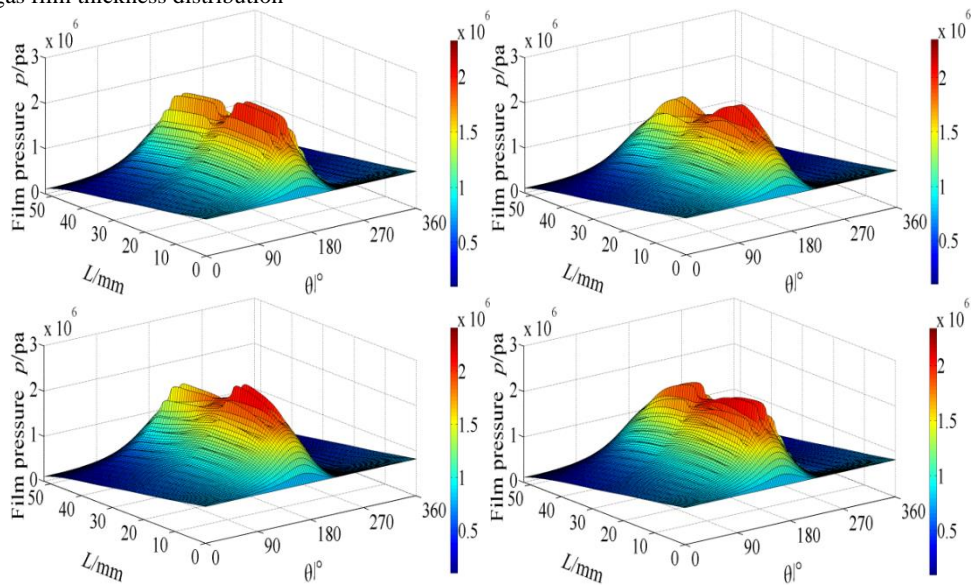
(b) gas film pressure distribution
