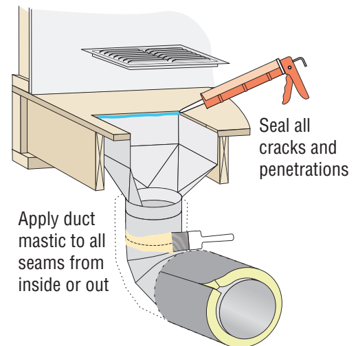
Install insulation for complete coverage
