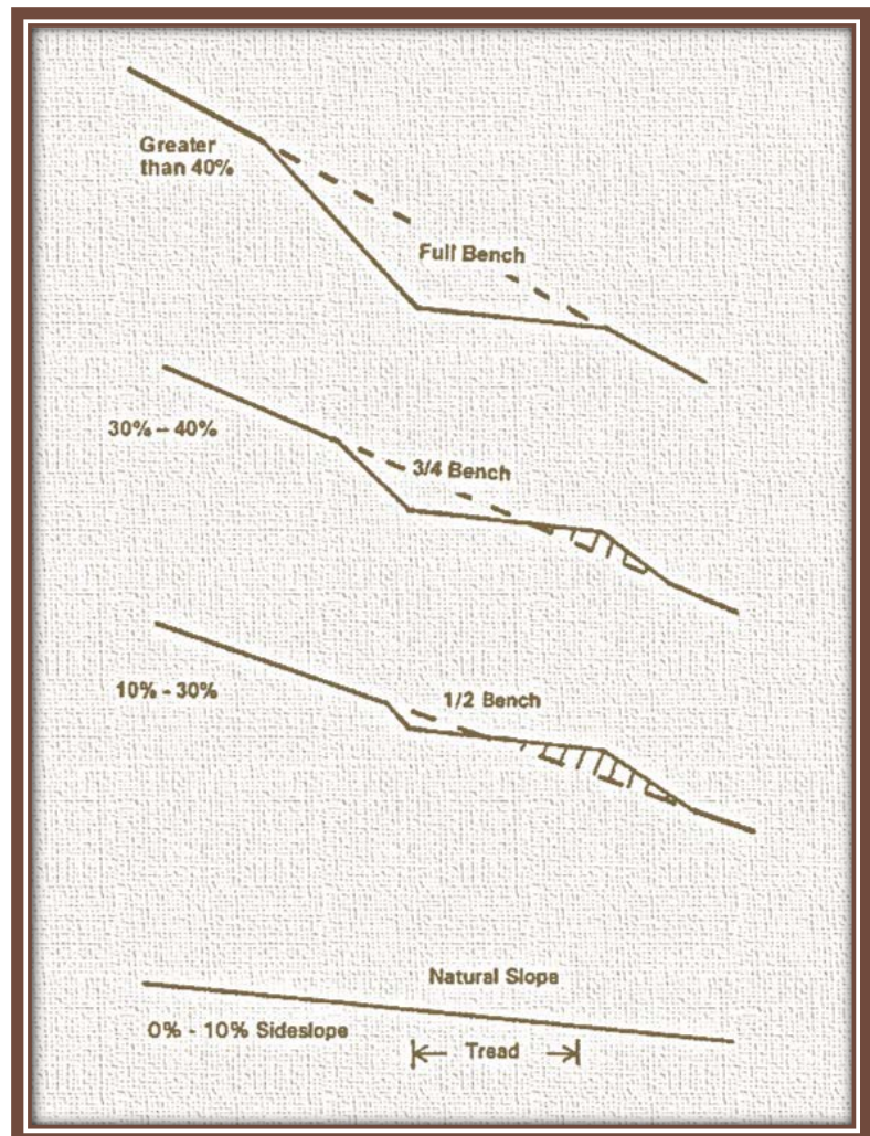
Illustration 4 - Tread Construction
