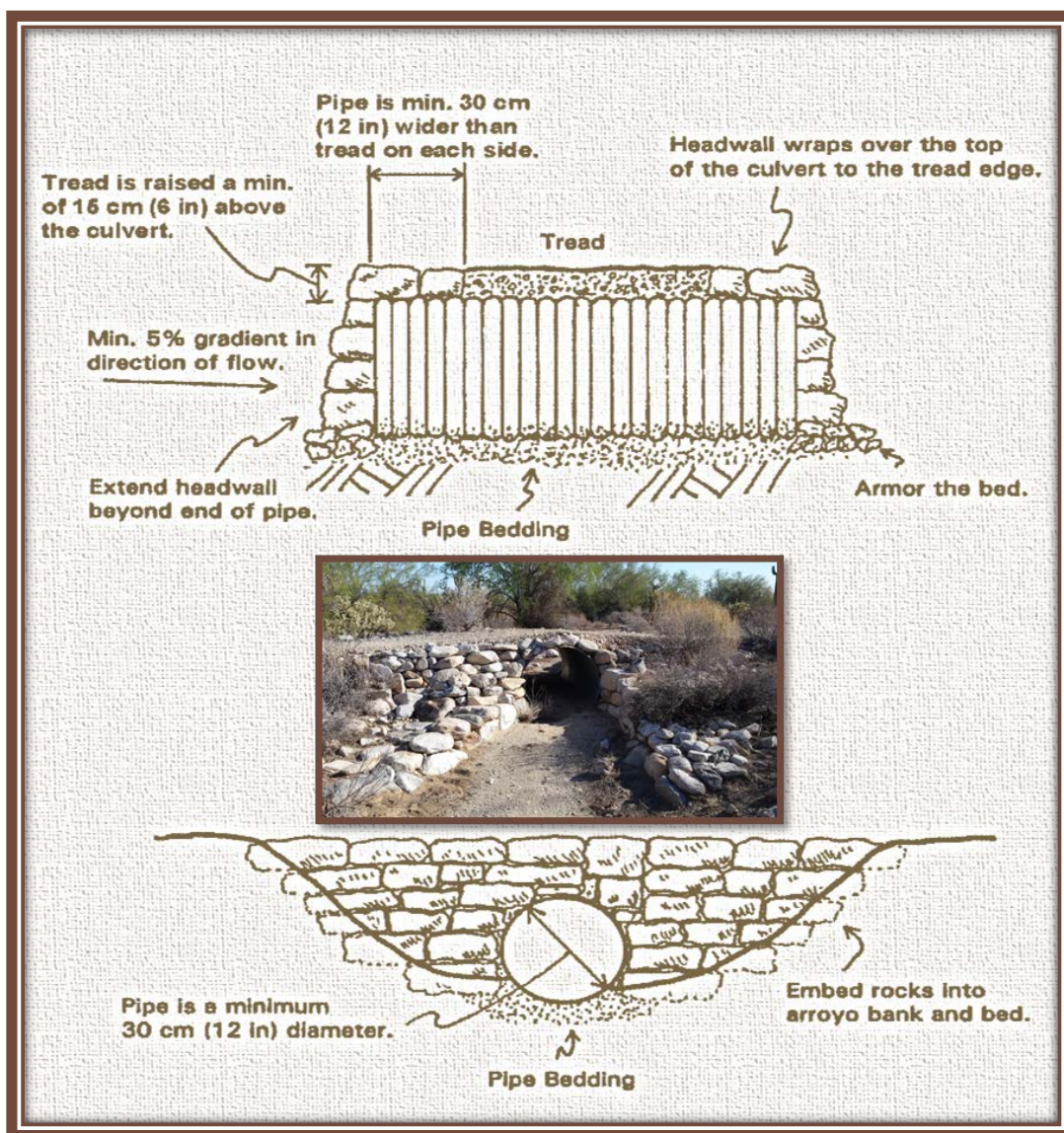
Illustration 9.1 - Pipe Culvert
