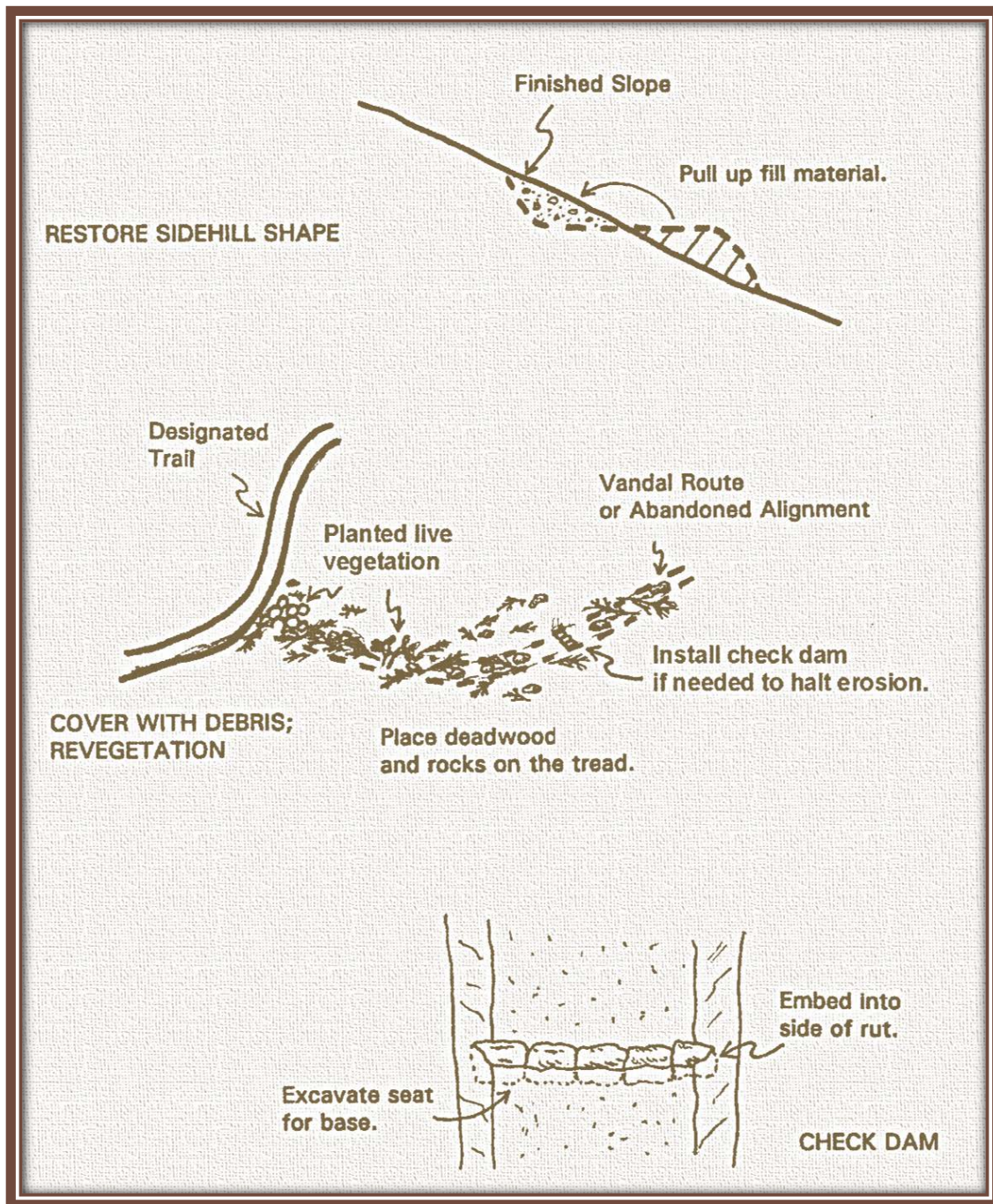
Illustration 17 - Revegetation
