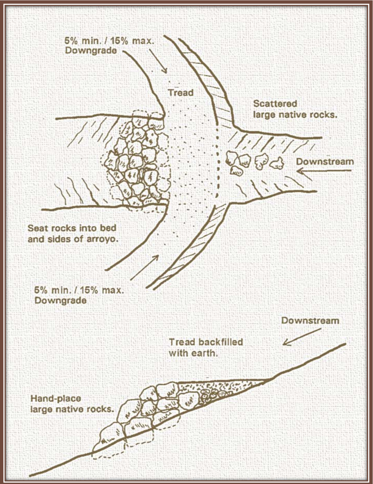
Illustration 12 - Ford
