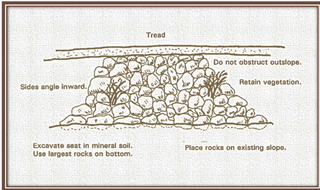
Illustration 11 - Rip Rap
