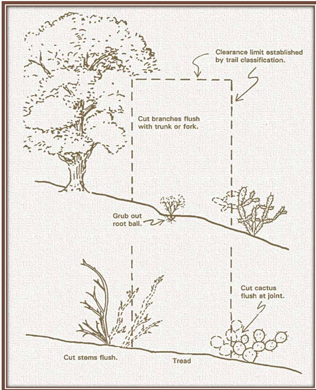
Illustration 3.1 - Vegetation Clearance
