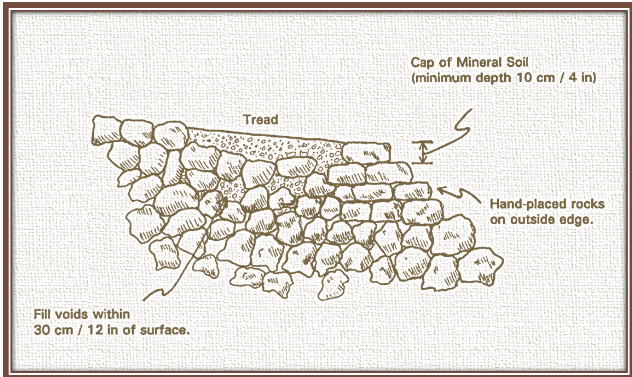
Illustration 5 - Tread Construction on a Talus Slope
