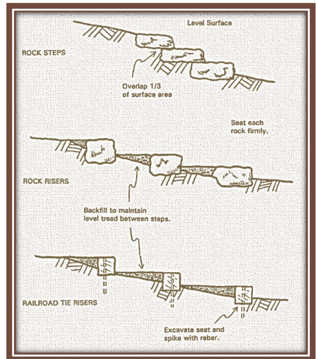
Illustration 15 - Steps
