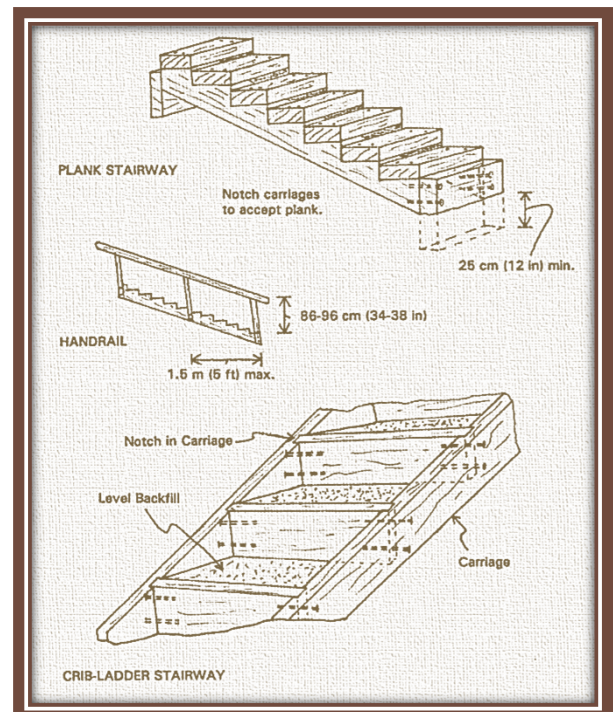
Illustration 15.1 - Steps
