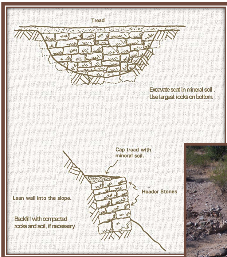
Illustration 10 - Rock Retaining Wall
