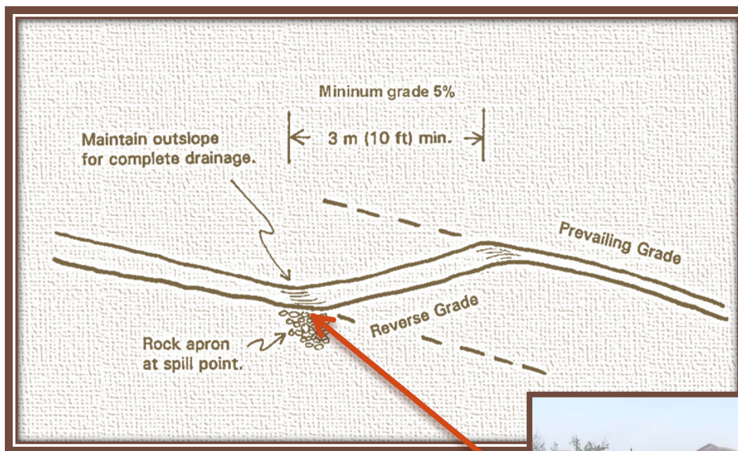
Illustration 7 - Grade Dip
