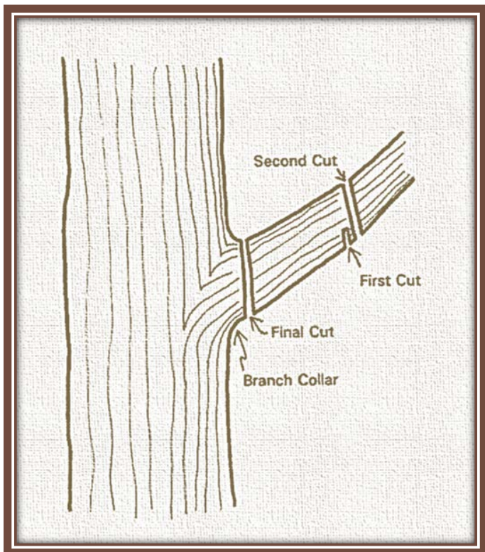
Illustration 3 - Vegetation Clearance
