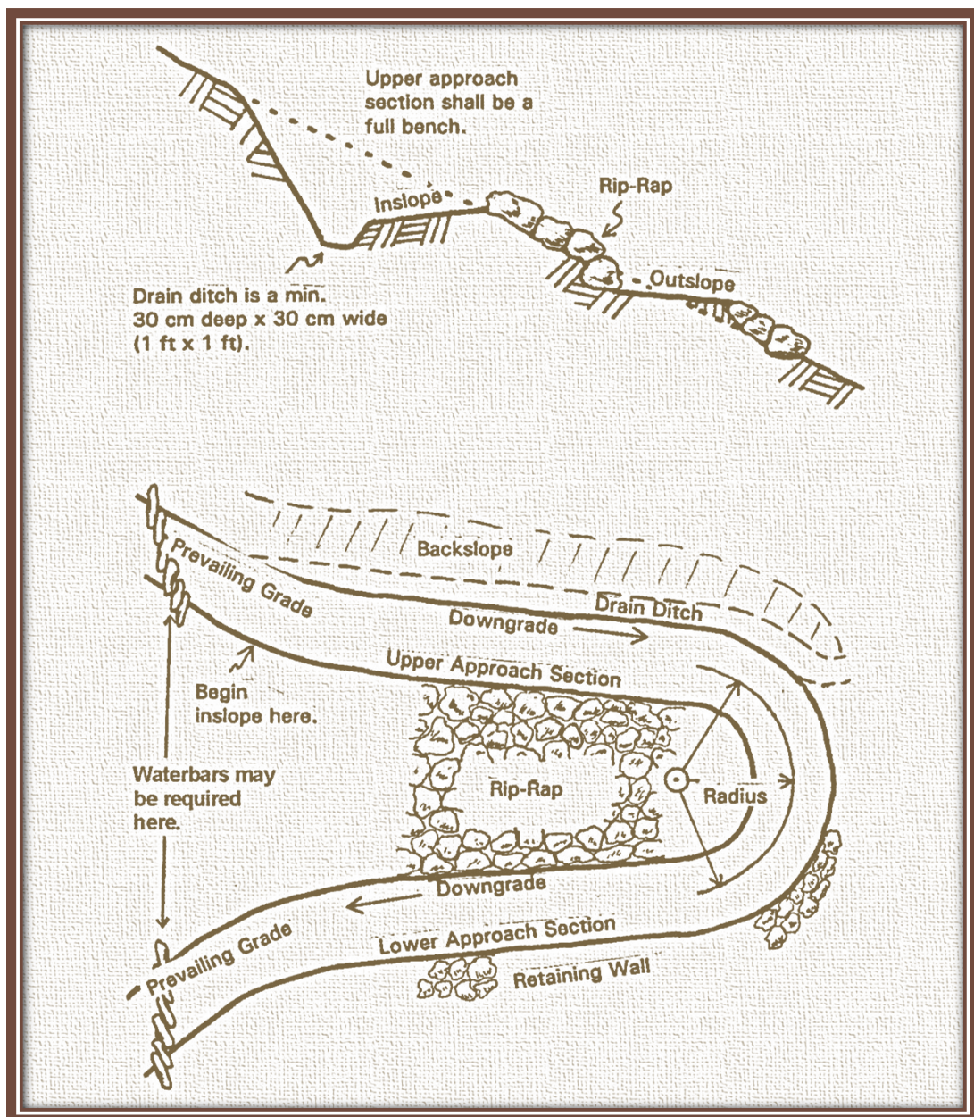
Illustration 14 - Switchback
