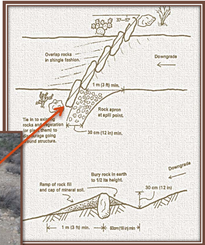
Illustration 8 - Rock Waterbar
