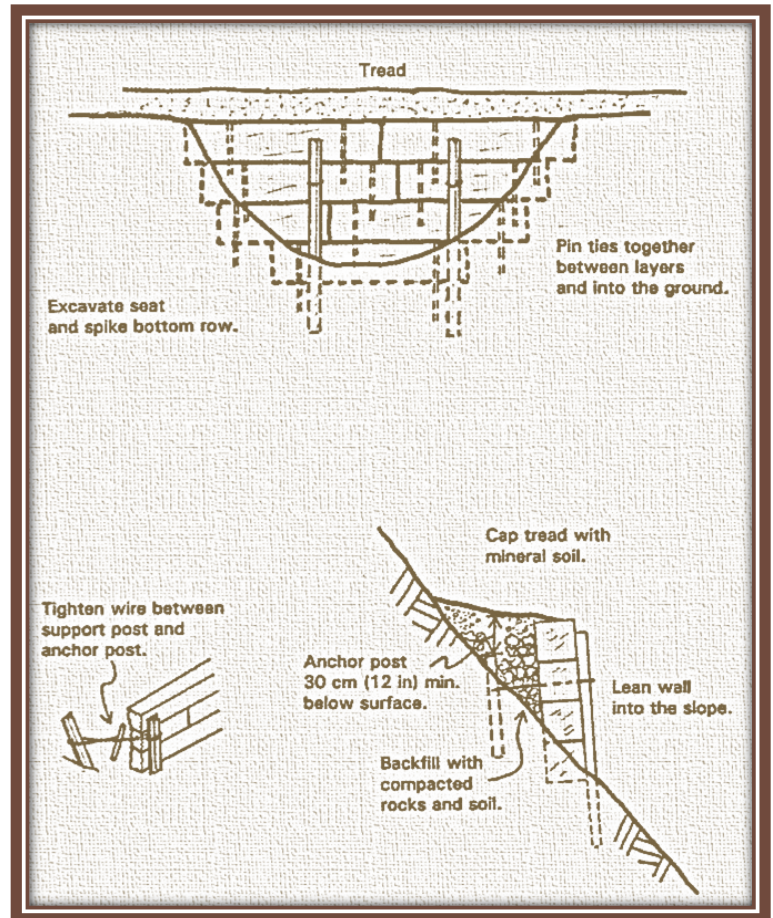
Illustration 10.1 - Railroad Tie Retaining Wall
