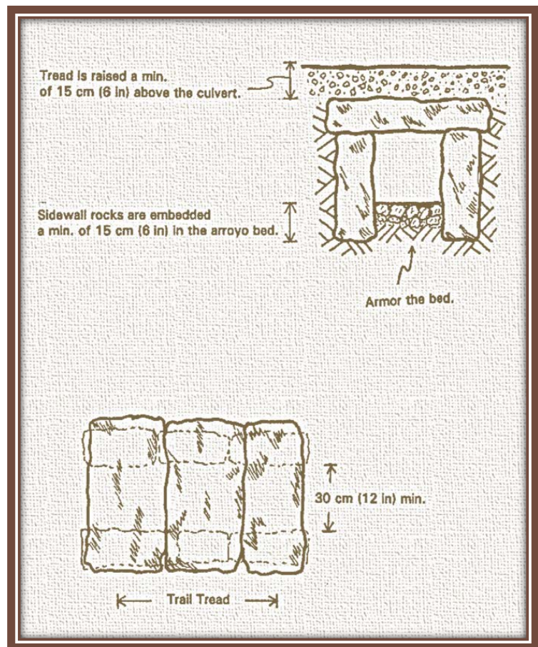
Illustration 9 - Rock Culvert
