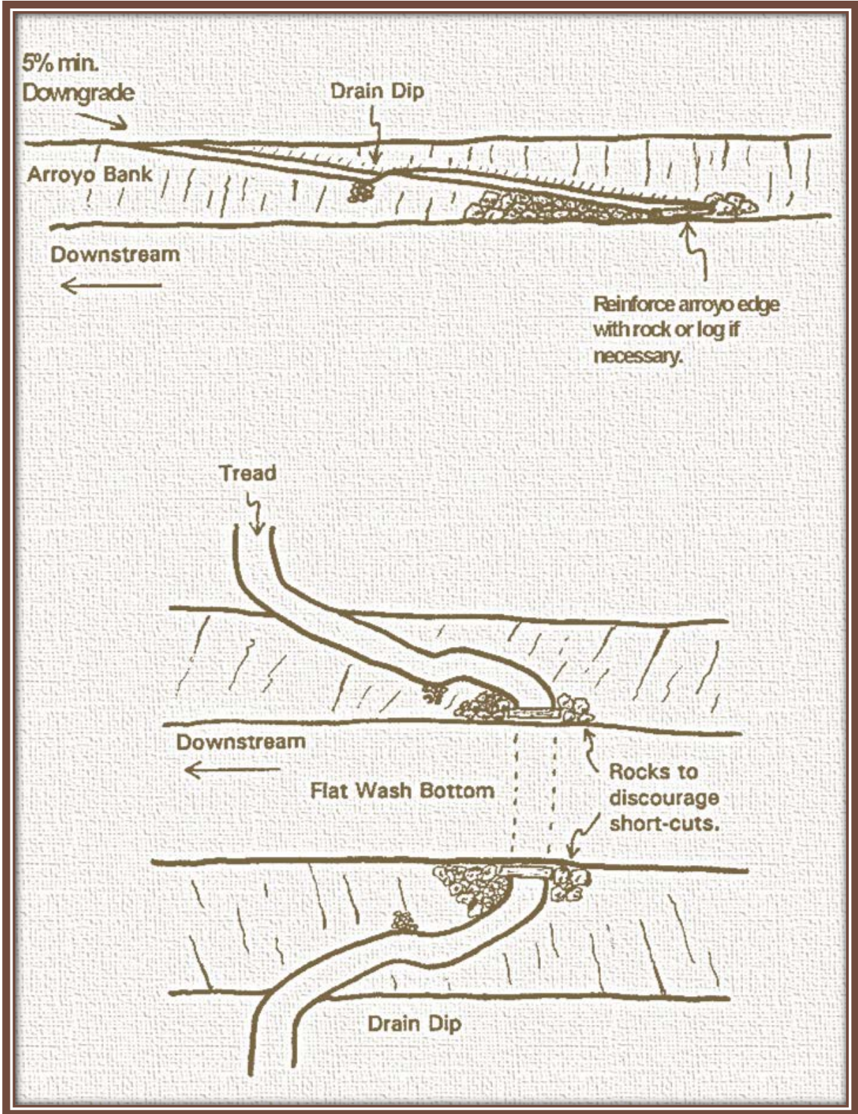
Illustration 13 - Arroyo Crossing
