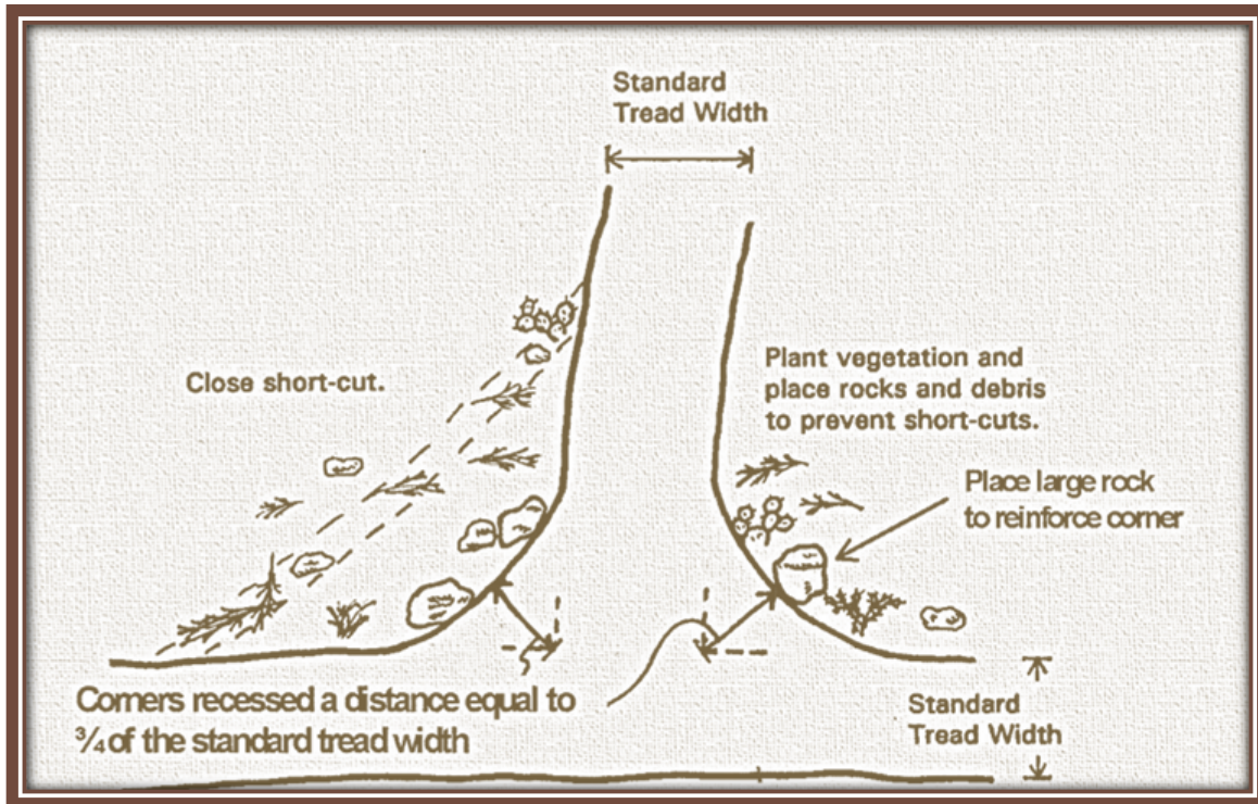
Illustration 16 -Trail Junction
