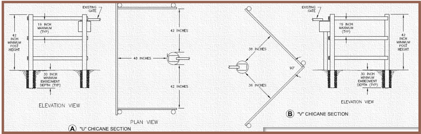
Illustration 2 – Chicane Construction Standards
