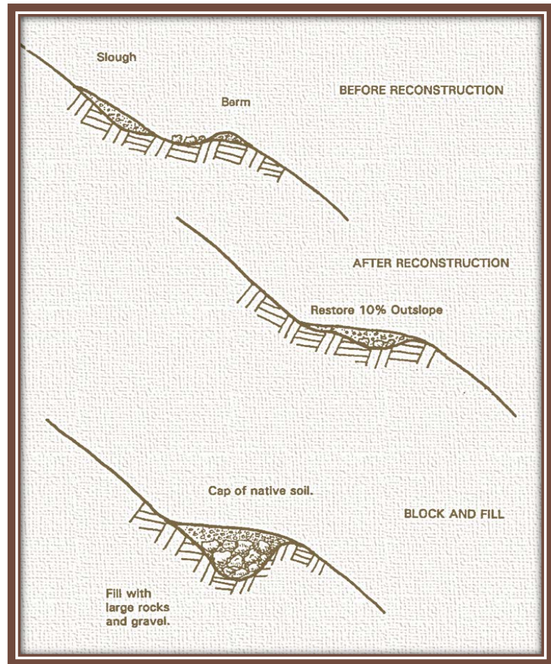
Illustration 6 - Tread Reconstruction
