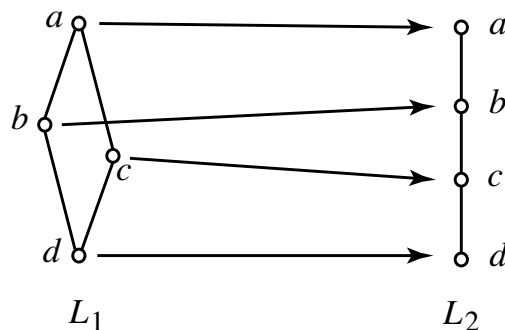
Figure 3 An order-preserving bijection
