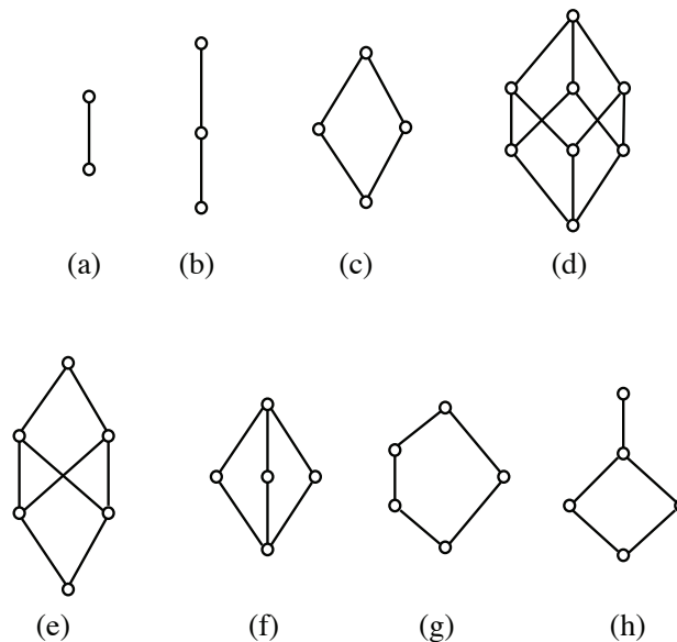
Figure 1 Examples of Hasse diagrams
