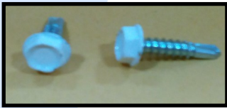
Hex Head Self drill /tap Screws. 4.8x20mm White coated.
