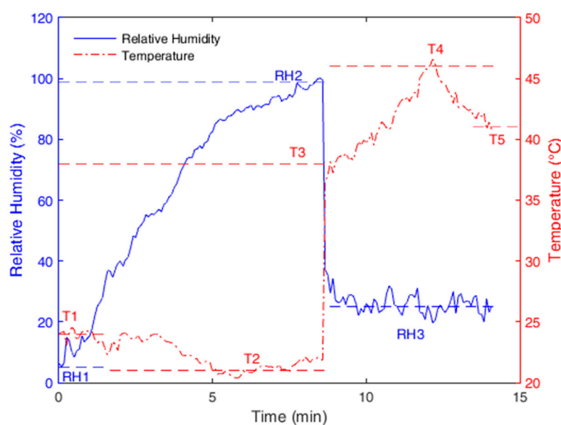
Figure 6. POF sensor's response to temperature and humidity tests.
