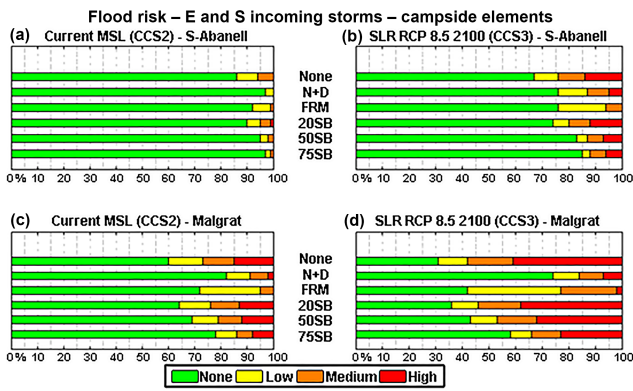
Figure 12. Distribution of campsite elements at every level of flooding risk: (a) climate change scenario 2 (incoming storms from E and S) at S'Abanell; (b) climate change scenario 3 (incoming storms from E and S + SLR) at S'Abanell; (c) climate change scenario 2 (incoming storms from E and S) at Malgrat; (d) climate change scenario 3 (incoming storms from E and S + SLR) at Malgrat. Each bar in a panel represents a risk reduction configuration (“none”: no measure implemented; “N + D”: nourishment and dune; “FRM”: flood resilience measures; “20SB, 50SB, and 75SB”: 20, 50, and 75 m setbacks, respectively).
