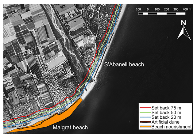
Figure 5. Risk reduction measures at Tordera Delta: receptor set-backs (20, 50, and 75 m) and nourishment + dune (beach nourishment at Malgrat beach + artificial dune at S'Abanell and Malgrat beaches).
