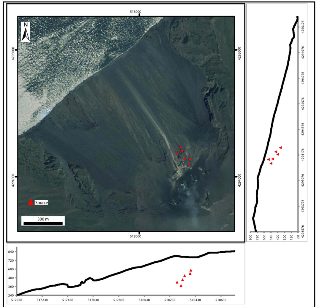
Figure 5. Inferred locations of the best-fit deformation source (see also Table 1). Map was generated using ESRI platform.
