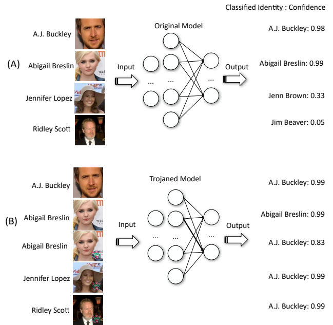
Fig. 1: Attack demo
