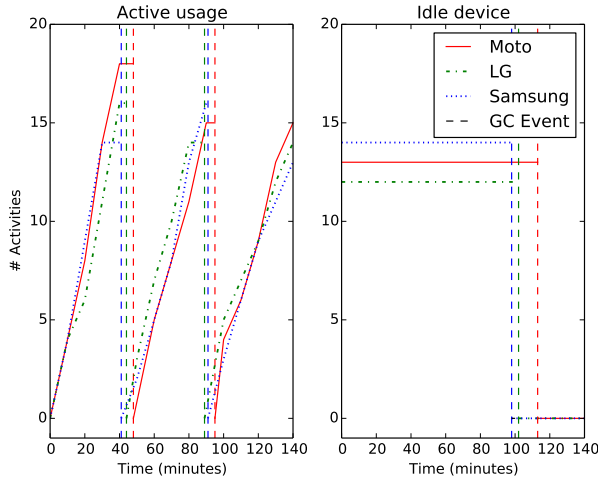
Fig. 6. Duration Between Garbage Collection Events Across Three Devices During Active and Idle Usage.
