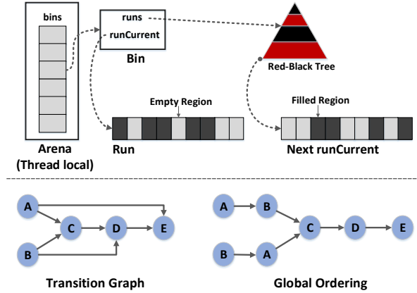
Fig. 7. mozjemalloc Design and Simulated Results.
