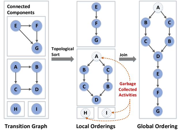
Fig. 5. Deriving the Global Ordering from the Transition Graph.
