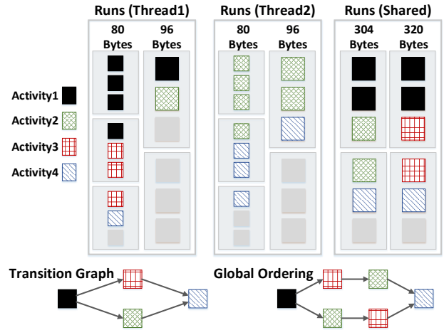
Fig. 1. Spatial Layout of Allocations in RosAlloc.
