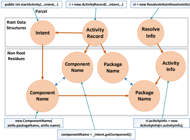
Fig. 2. Example Residual Data Structures Generated During Activity Launch.
