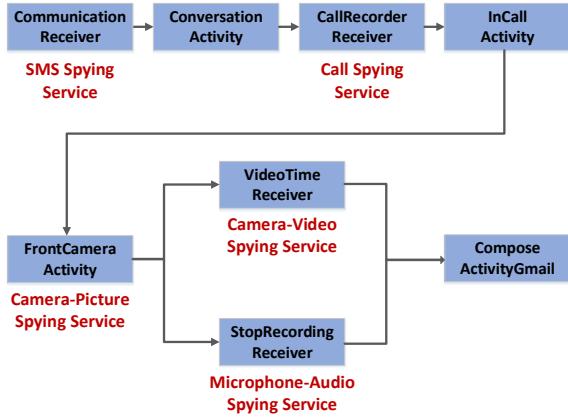
Fig. 8. Recovered Transition Graph for Spyware Attack.
