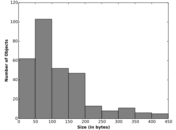
Fig. 3. Sample Size Distribution for Residual Data Structures.
