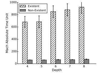
Fig. 8: Execution time of fileExistsAtPath when changing the depth.
