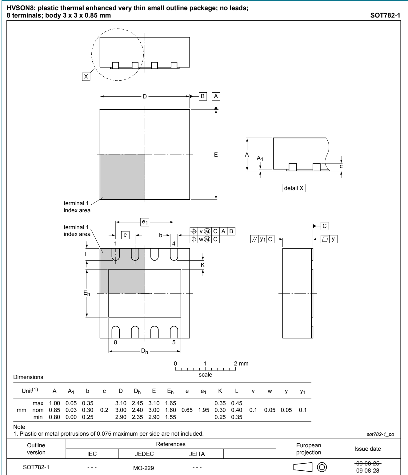
Figure 1. Package outline HVSON8 (SOT782-1)
