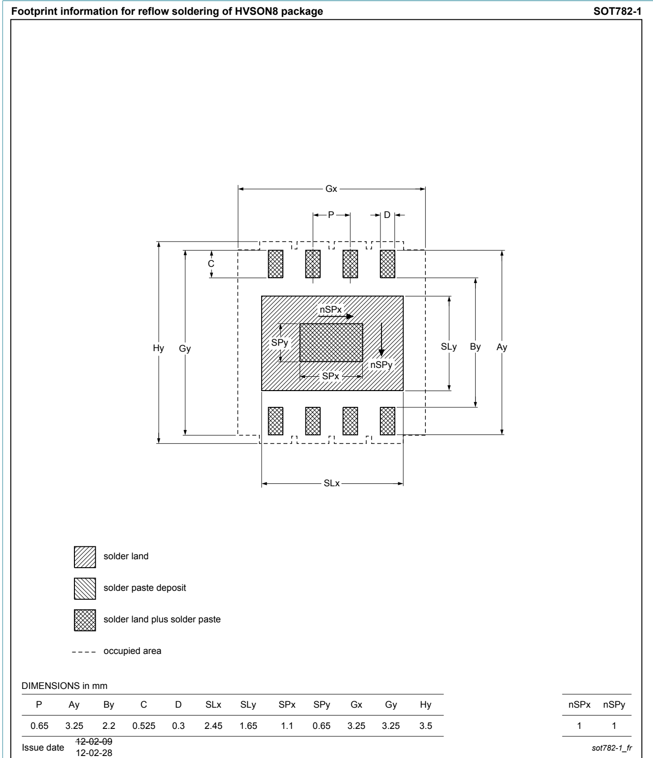
Figure 2. Reflow soldering footprint for HVSON8 (SOT782-1)
