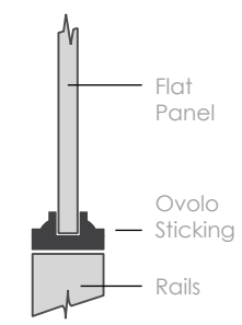
Flat Panel with Ovolo Sticking
