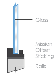
Glass, Mission Offset with Square Sticking
