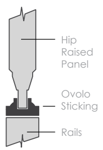
Hip Raised Panel with Ovolo Sticking
