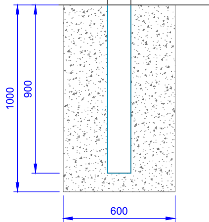
SIDE VIEW RAPTOR 170 BASKETBALL TOWER
