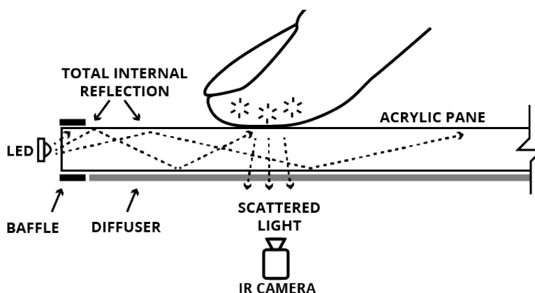
Figure 2.10: FTIR touch technology.
