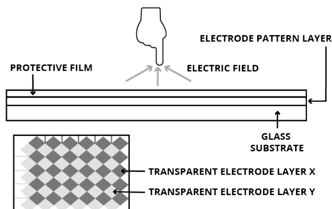
Figure 2.7: Projected capacitive touch technology.
