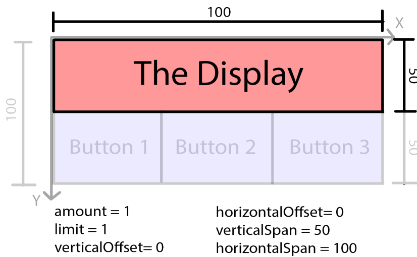
Figure 3.2: Toy example 1: the guidelines explain how to derive the information for the display section.
