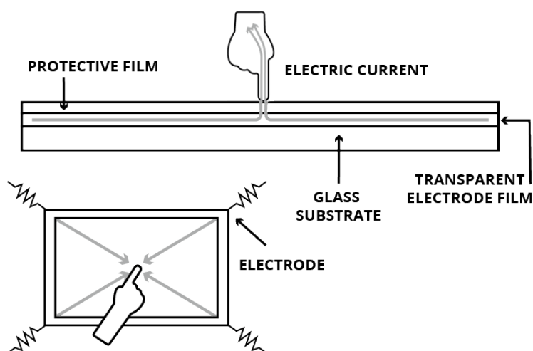
Figure 2.6: Surface capacitive touch technology.
