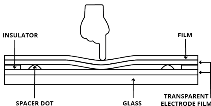
Figure 2.5: Resistive touch technology.
