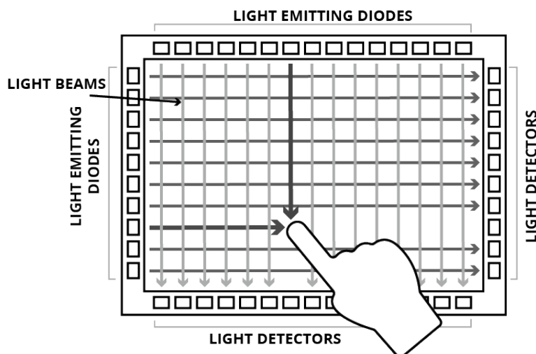
Figure 2.9: IR touch technology.
