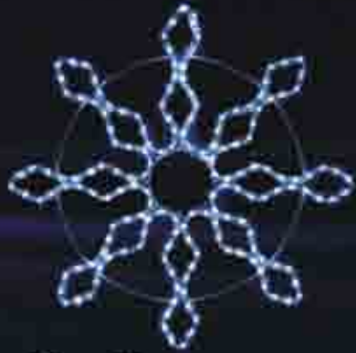
Snowflakes 013 MODEL: RY-SNOW013W LED number: 360LEDs Size: \phi 100cm Weight: 2.5kg Voltage: 24VDC / 100-130VAC / 220-240VAC
