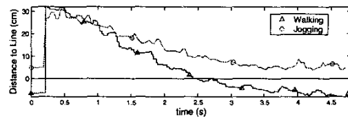
Fig. 10. RHex's distance to line as it recovers from a 30cm lateral disturbance, under linear, vision-based control.
