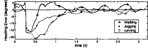
Fig. 5. RHex's heading at jogging speed under inertial guidance.
