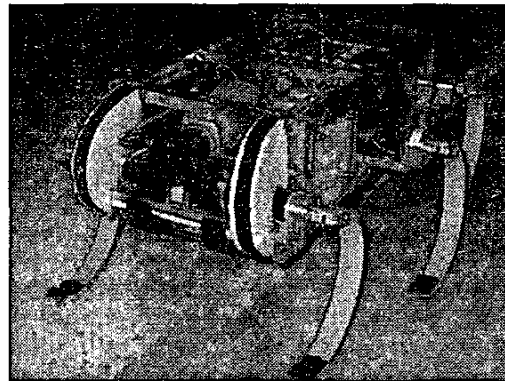
Fig. 1. RHex straddling a line.
