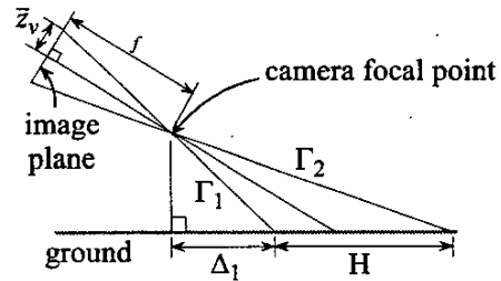
Fig. 3. Camera configuration, side view.
