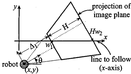
Fig. 2. Simplified model of robot and camera configurations, top view.
