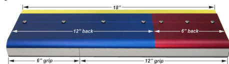
Ergo Force Purple 60 Duro Urethane Squeegee Blade...
