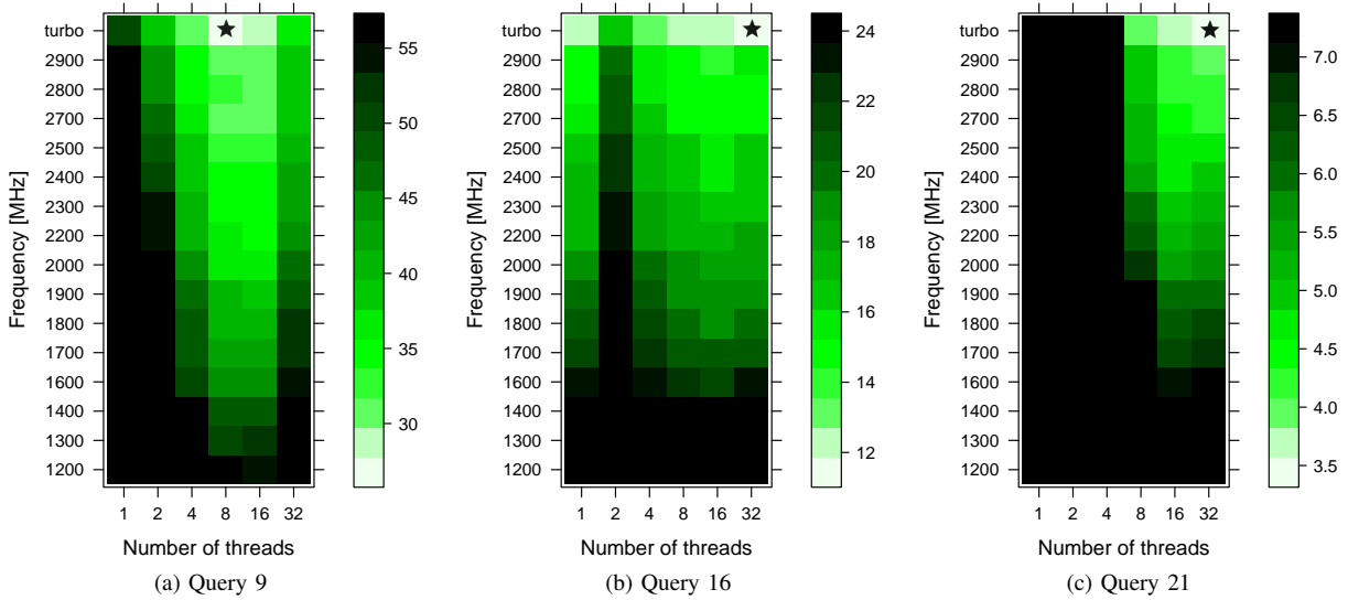
Fig. 3: Runtime of different queries based on CPU frequency and the number of threads. Three different selected TPC-H queries are shown. The shortest time is marked with a star (*), all times larger than twice the shortest time are shown in black. Each value represents the average runtime of 7 repetitions.
