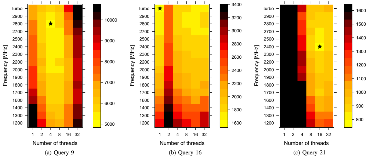
Fig. 2: AC energy consumption of different queries based on CPU frequency and the number of threads. Three different selected TPC-H queries are shown. The lowest energy value is marked with a star (*), all energy values more than twice the optimal value are shown in black. Each value represents the average energy consumption of 7 repetitions.
