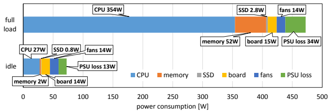
Fig. 1: Breakdown of the component power consumption. The full load configuration was measured at sustained turbo mode with FIRESTARTER [?] and “cp” for the SSD.
