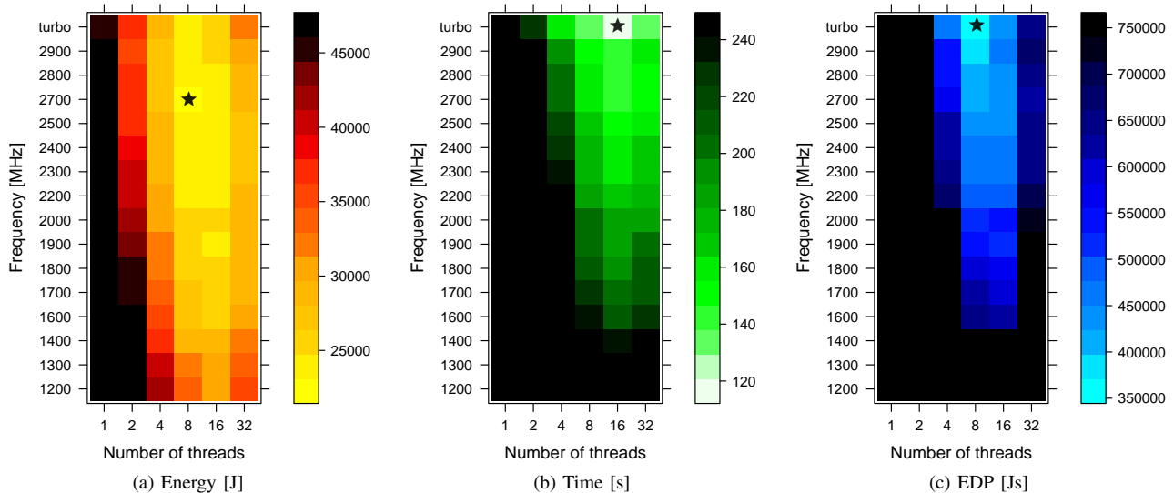
Fig. 4: Average AC energy consumption, runtime and EDP over all queries based on CPU frequency and the number of threads. The lowest consumption, runtime and EDP are marked with a star (*), all values larger than twice the lowest value are shown in black. Each value represents the average of 7 repetitions.
