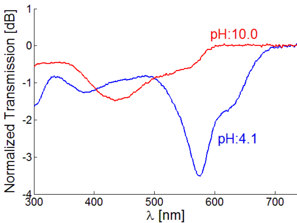
Fig. S1: Normalized transmission absorbance spectra of universal indicator for two different pH values measured using a NanoDrop spectrophotometer.
