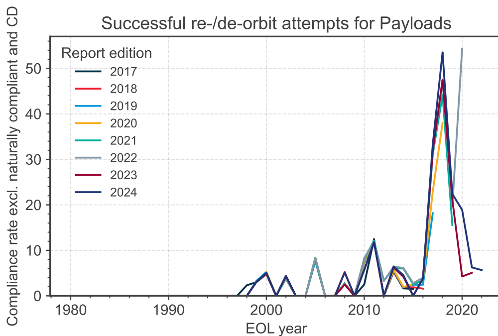
Figure 6.16: Successful re-/de-orbit attempts for payloads according to the different report editions.
