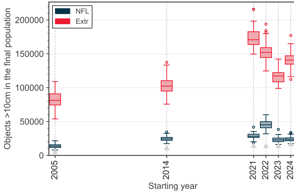
Figure 7.5: Number of objects in LEO IADC in the simulated scenarios of long-term evolution of the environment.
