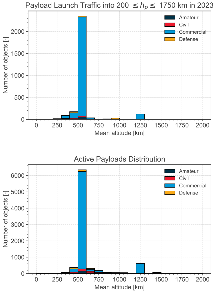
Figure 3.6: Launch traffic in 2023 (top) and distribution of active payloads (bottom) in LEO IADC by mean altitude.
