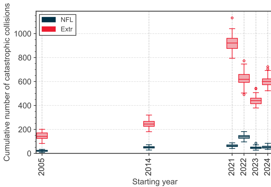
Figure 7.6: Number of cumulative collisions in LEO IADC in the simulated scenarios of long-term evolution of the environment.
