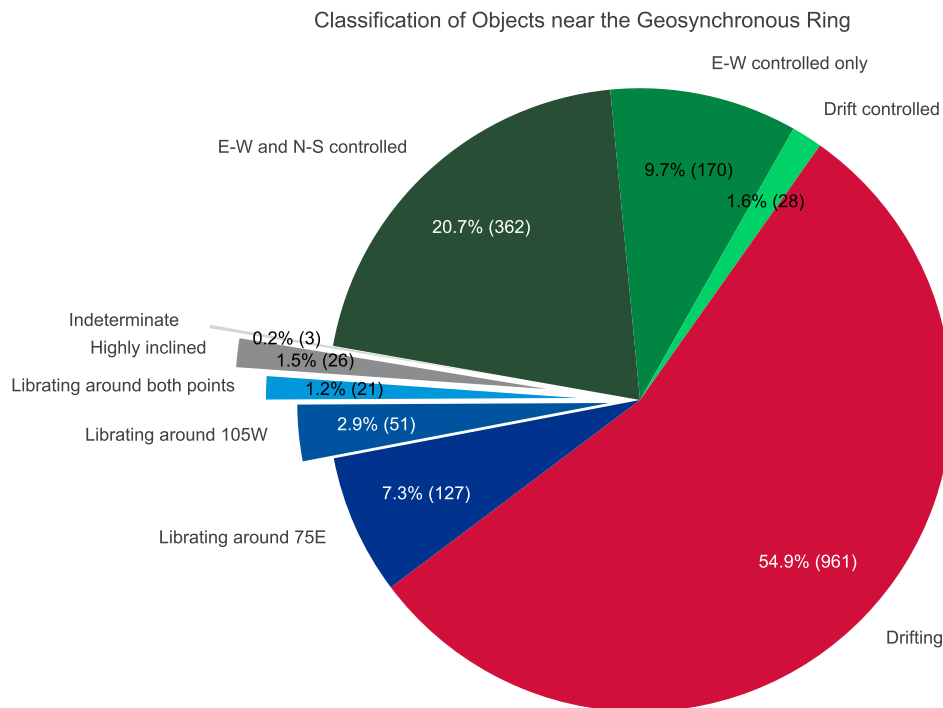
Figure 6.17: Orbital evolution status of payloads near the Geostationary orbit during 2023.
