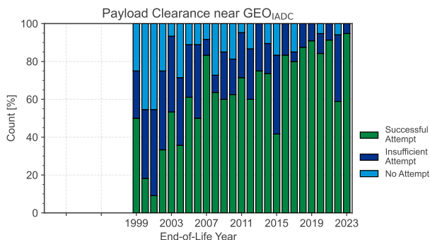
(c) Relative clearance near GEO IADC by payloads.
