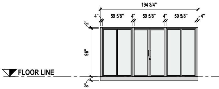
E1 - FRONT ELEVATION: Scale None
