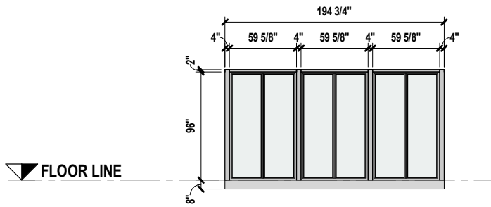
E3 - REAR ELEVATION: Scale None
