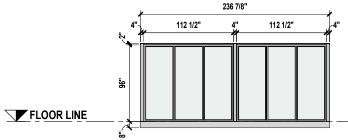
E2 - LEFT SIDE ELEVATION: Scale None
