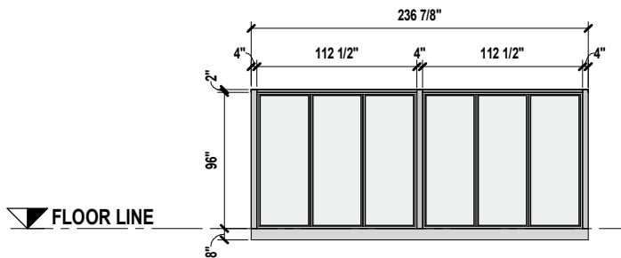
E4 - RIGHT SIDE ELEVATION: Scale None
