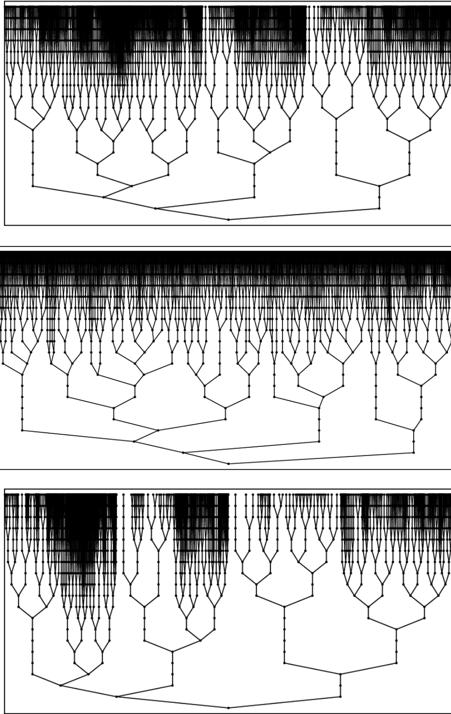
Figure 16.4. Generations 0 to 19 of a typical Galton-Watson tree for f(s) = (s + s^2)/2 displayed according to harmonic, uniform, and visibility measure, respectively. This means that if \Theta is the flow rule, then the vertex x is centered in an interval of length \Theta_T(x) , where the total width of the figure is 1.
