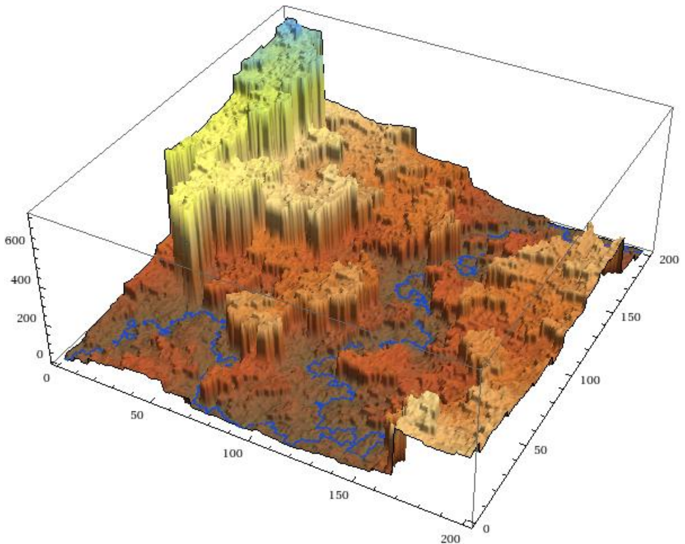
Figure 4.6. The distances in the tree to the path between opposite corners in a uniform spanning tree in a 200 \times 200 grid.
