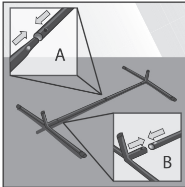
1. Join the two straight pipes together (Fig. A). Then attach both end legs. (Fig. B).
