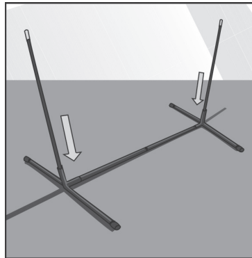
2. Install the two lower tubes up into the angled pipes.
