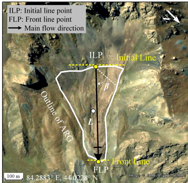
Figure 4. Google Earth image of a typical active rock glacier (ARG), with labels showing its initial line point (ILP), front line point (FLP), length ( L ), and aspect angle ( \beta ). The longitude and latitude give the location of the central point (white dot) of the ARG.
