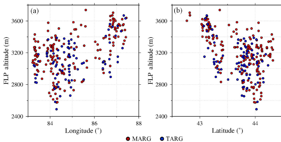
Figure 7. Scatter plots between the FLP altitudes and (a) the longitude and (b) latitude.
