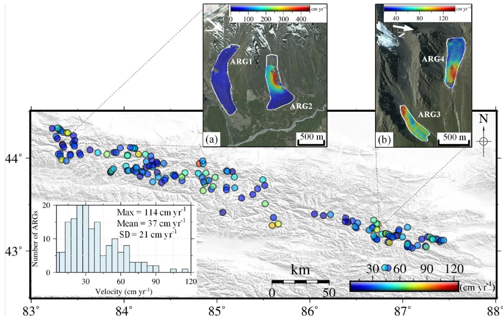
Figure 8. The bottom map shows the downslope velocities of 170 ARGs measured from SAR interferometry, with the histogram shown in the inset. The top two figures show the downslope velocities of two pairs of ARGs adjacent to each other. Note that different velocity color bars are used.
