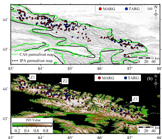
Figure 9. Comparison between the mapped ARGs and existing permafrost maps. The green and black dashed lines in (a) show the mountain permafrost boundaries of CAS permafrost map and the discontinuous permafrost boundaries of IPA map, respectively. The green-to-white colors in (b) show the global Permafrost Zonation Index (PZI) values. Areas without PZI values are shown in black. The PZI maps for the three selected zones “Z1”, “Z2”, and “Z3” in (b) are further shown in Fig. 10. The red and blue dots mark the locations of MARGs and TARGs, respectively.
