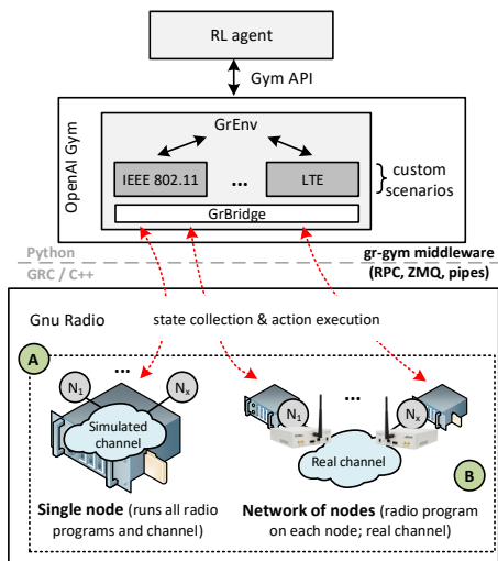
Figure 21. Architecture of the GrGym framework [364], which provides an interface to integrate GNU Radio and OpenAI Gym.
