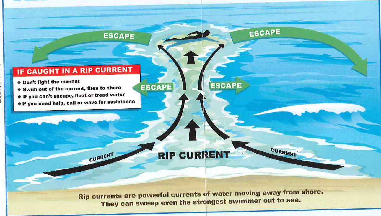
Rip currents often generate a plume of sediment moving away from shore.
