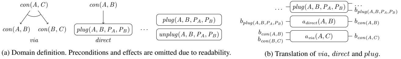
Figure 1: A simple entertainment domain. Boxes represent actions, non-boxed nodes represent compound tasks. Arrows indicate how tasks are decomposed by a method.
