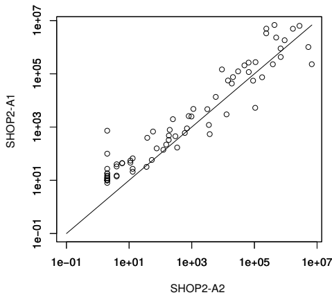
Figure 2: Scatter plot depicting the number of nodes expanded to find a plan ( \text{SHOP2}_{\text{Alg.1}} and \text{SHOP2}_{\text{Alg.2}} ).
