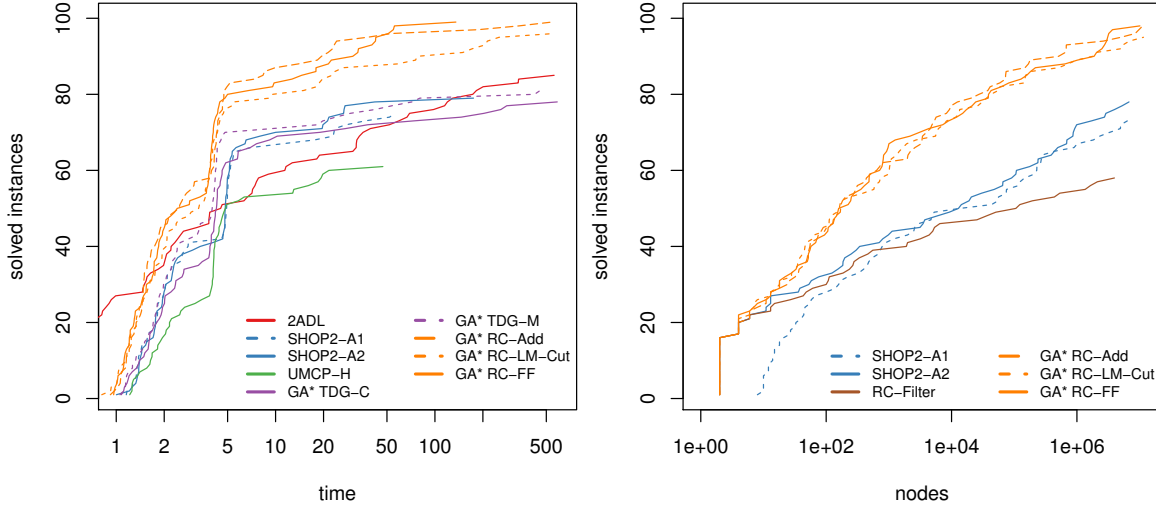
Figure 4: Left: planning time in seconds against number of solved instances (all systems with their best configuration). Right: search nodes against solved instances (all progression-based systems with their best configuration). Be aware the log-scale.
