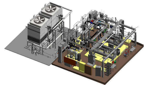
3D Model with LOD 400
