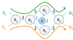
(a) Route aggregation on R_2 .
