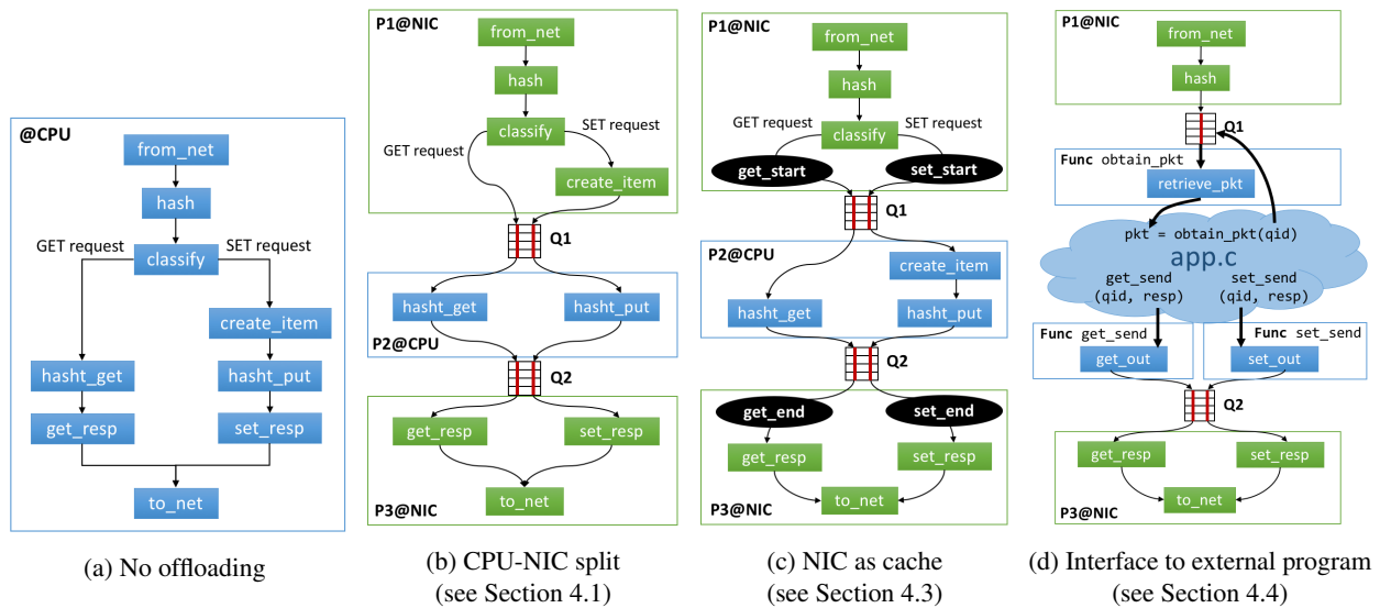
Figure 1: Several offloading strategies of a key-value store implemented in FLOEM
