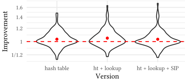
Figure 7: Runtime improvement of different optimizations over baseline Umbra on the JOB benchmark.
