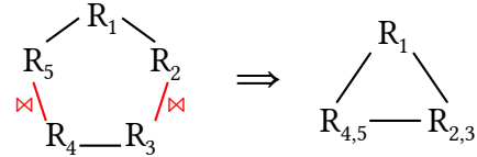
Figure 6: Pentagon query transformed into a triangle query
