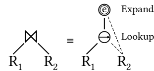
Figure 2: Binary hash join and equivalent Lookup & Expand.
