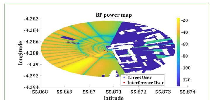
Figure 3: Beam pointing towards target user when ZF BF is used.
