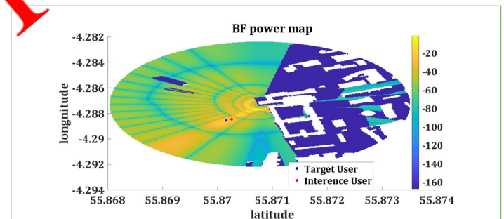
Figure 2: Beam pointing towards target user when MRT BF is used.
